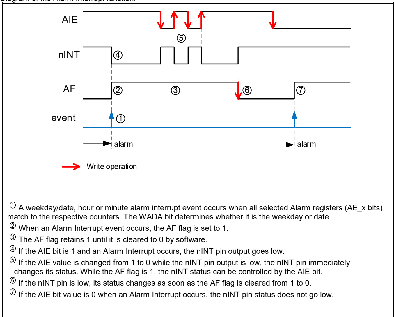
Figure 7-15 Alarm Interrupt
