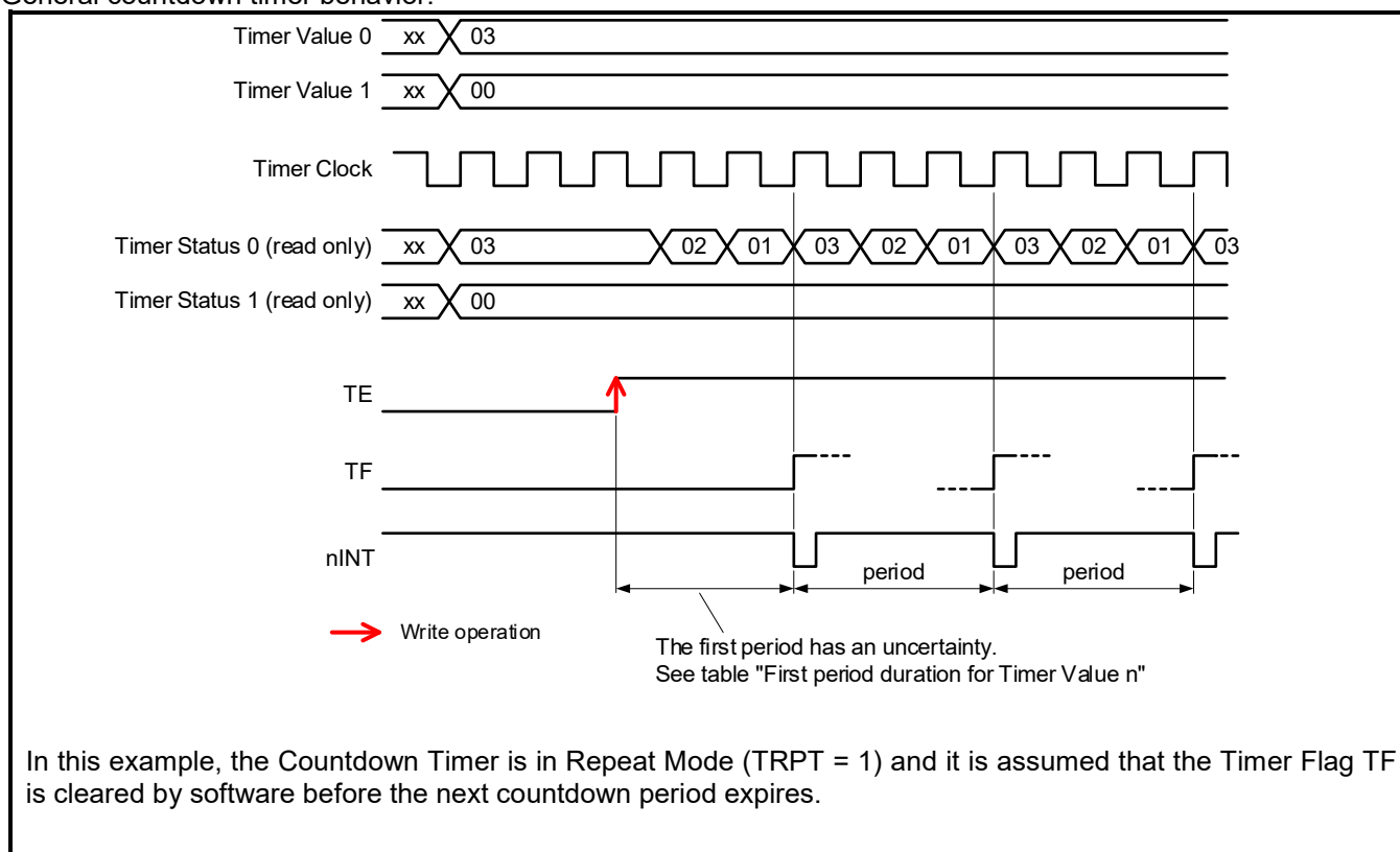
Figure 7-12 Periodic Countdown Timer Interrupt
