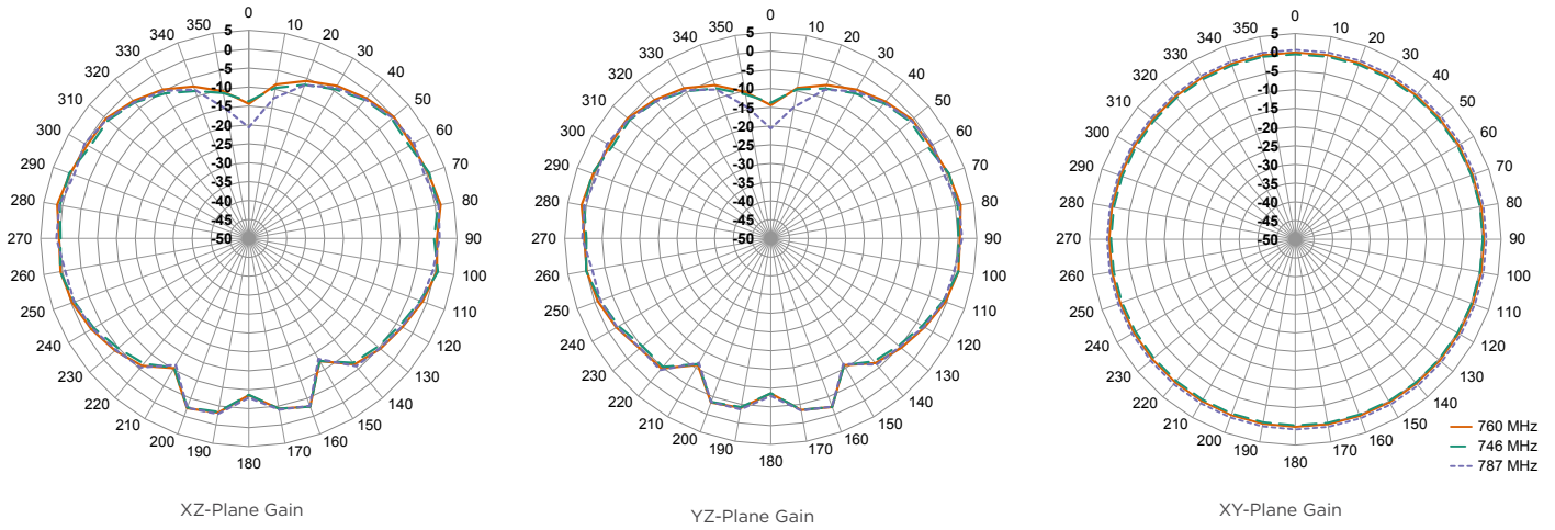
Figure 9: Radiation Patterns for CW LTE Band 13 Antenna
