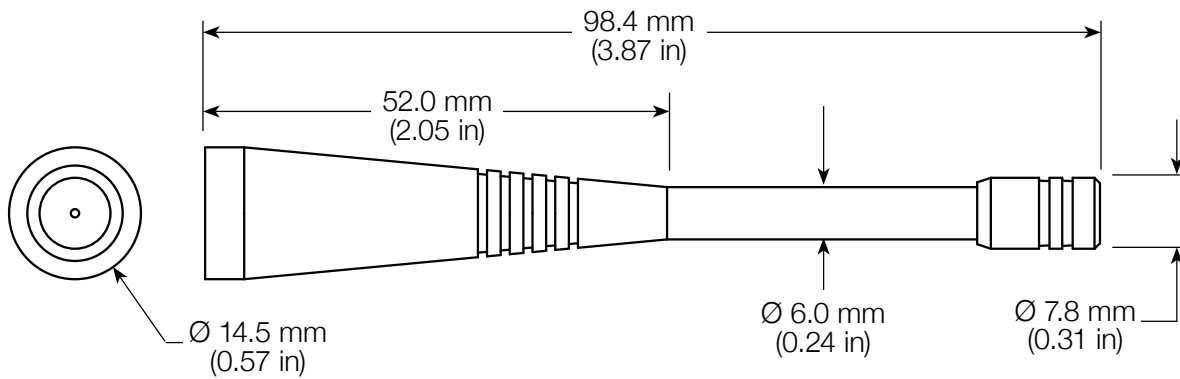
Figure 7: CW LTE Band 13 Antenna Dimensions
