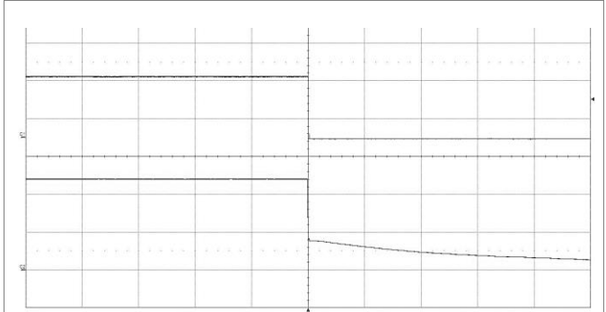
Output disabled by removing V_I at: T_{P1} = +25^{\circ}\text{C} , V_I = 24\text{ V} , I_O = 7\text{ A} resistive load. Top trace: output voltage (2 V/div.). Bottom trace: input voltage (10 V/div.). Time scale: (200 ms/div.).
