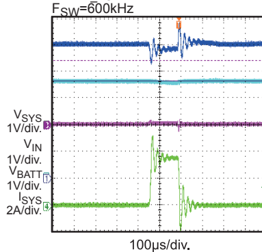
System Short Protection Zoom In
