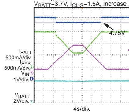
Input Voltage Clamp @ 4.75V Charge Mode
