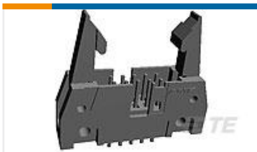
TE Part #5499206-9 A/L UNIV HDR 40P VERT LG LAT
