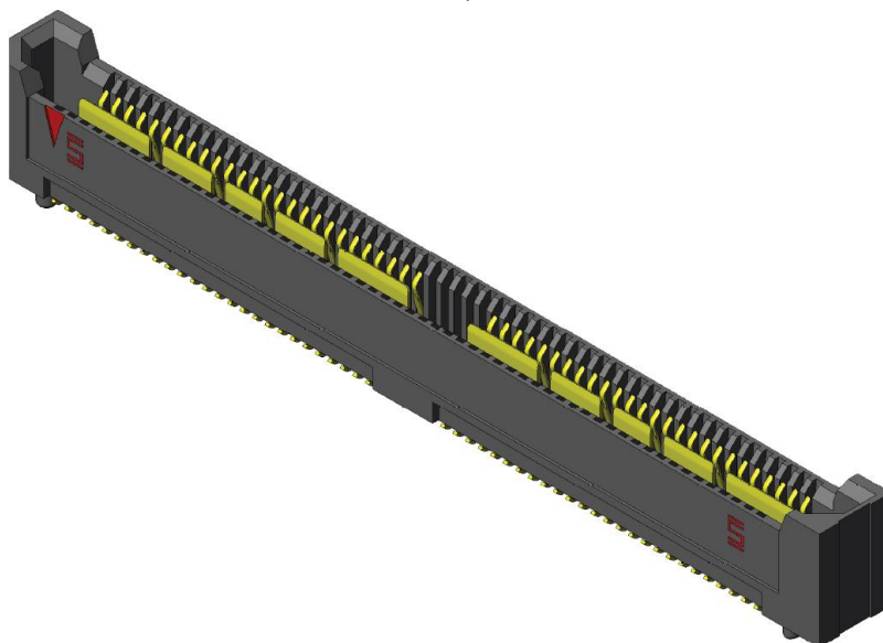
QRF8 Series – Socket, Vertical Orientation
