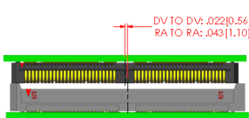
INITIAL X AXIS LINEAR MISALIGNMENT
