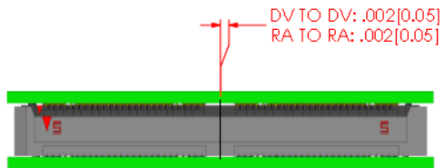
FINAL X AXIS LINEAR MISALIGNMENT
