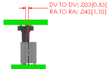
INITIAL Y AXIS LINEAR MISALIGNMENT
