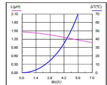
SMS0420-1R5M
