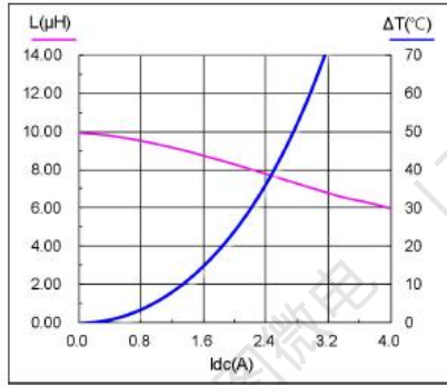
SMS0420-100M
