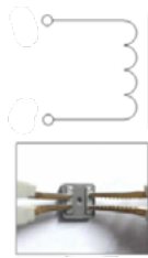
Figure 1. DCR test
