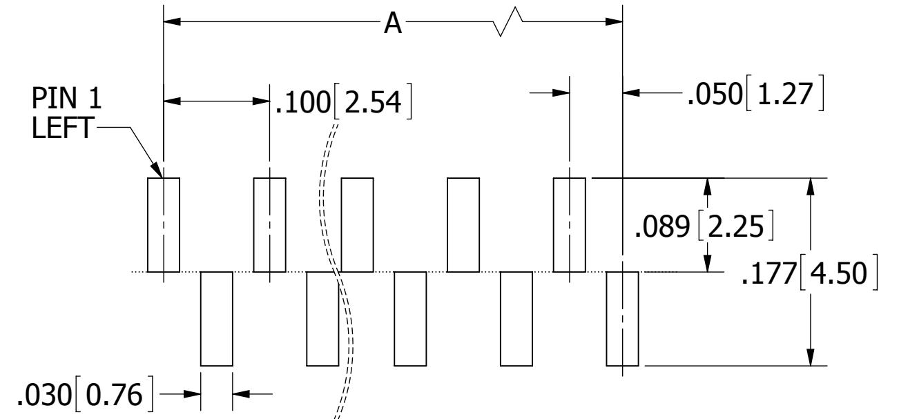
RECOMMENDED PCB LAYOUT GRP_1VWTC-RC
