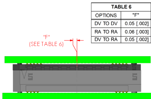
FINAL X AXIS LINEAR MISALIGNMENT
