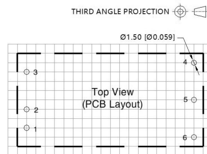
Note: Grid 2.54*2.54mm
