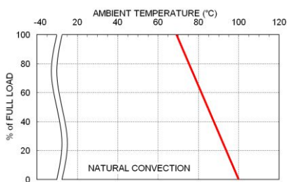
FKC08-48S05 Derating Curve
