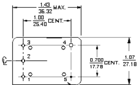
(VIEW FROM BOTTOM) NUMBERS FOR REFERENCE ONLY (NOT STAMPED ON UNIT)
