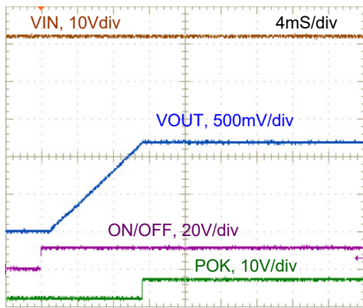
Figure 25. On/Off Enable wave form
