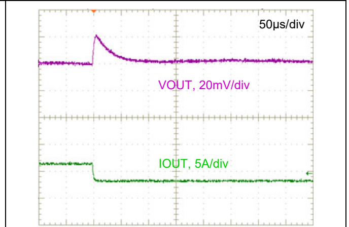
( V_{IN}=12V , C_{OUT}=200\mu F , I_{OUT}=6 to 3A , 1.0A/\mu s ) Figure 34. Step Load Transient Response
