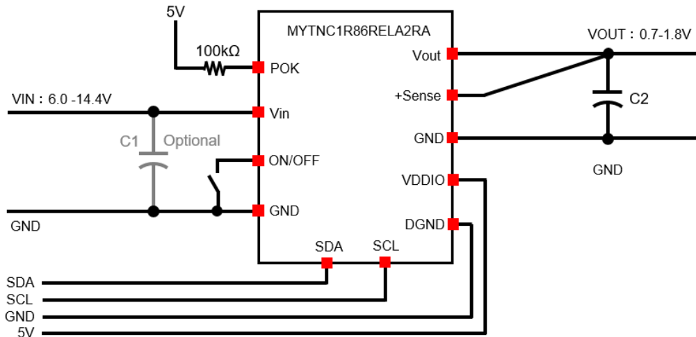
Figure 39. Application Schematic
