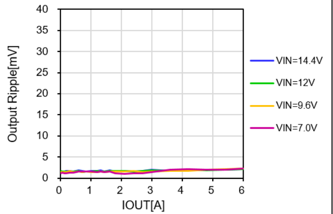
Figure 26. Output Ripple and Noise
