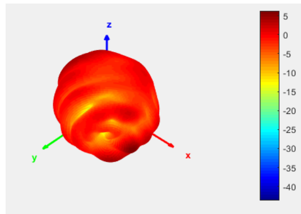
Radiation Pattern at 7.5GHz
