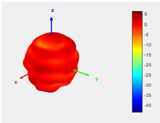
Radiation Pattern at 6.5GHz
