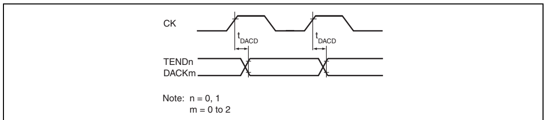
Figure 33.39 DACK, TEND Output Timing
