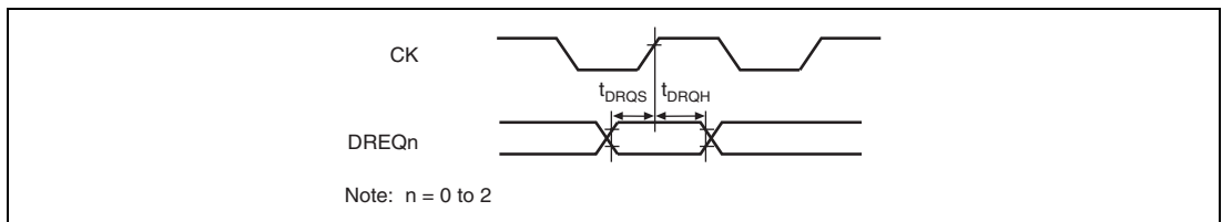
Figure 33.38 DREQ Input Timing
