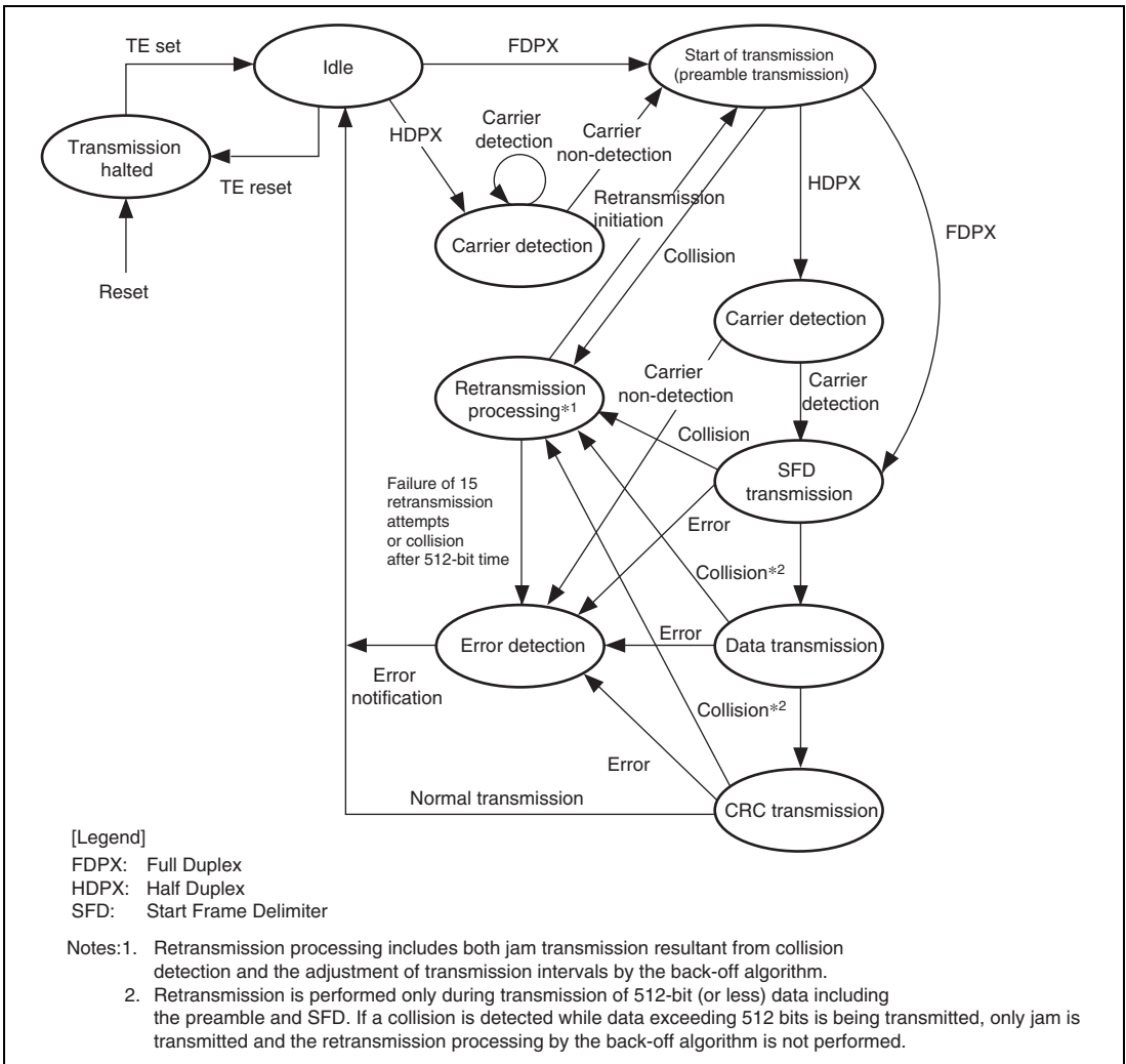
Figure 25.2 EtherC Transmitter State Transitions
