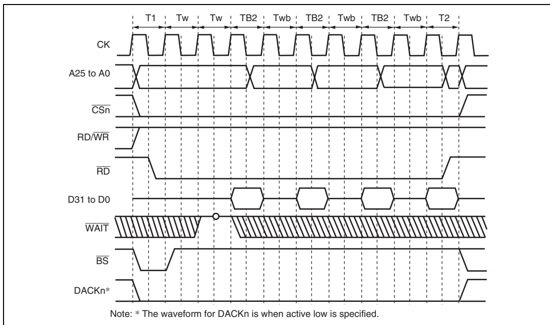
Figure 9.36 Burst ROM Access Timing (Clock Asynchronous) (Bus Width = 32 Bits, 16-Byte Transfer (Number of Burst 4), Wait Cycles Inserted in First Access = 2, Wait Cycles Inserted in Second and Subsequent Access Cycles = 1)
