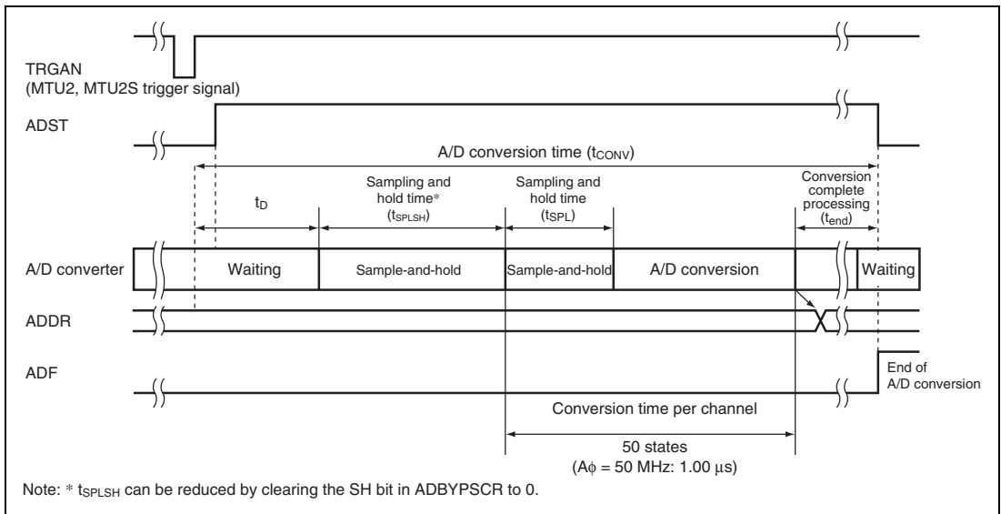
Figure 20.6 A/D Conversion Timing
