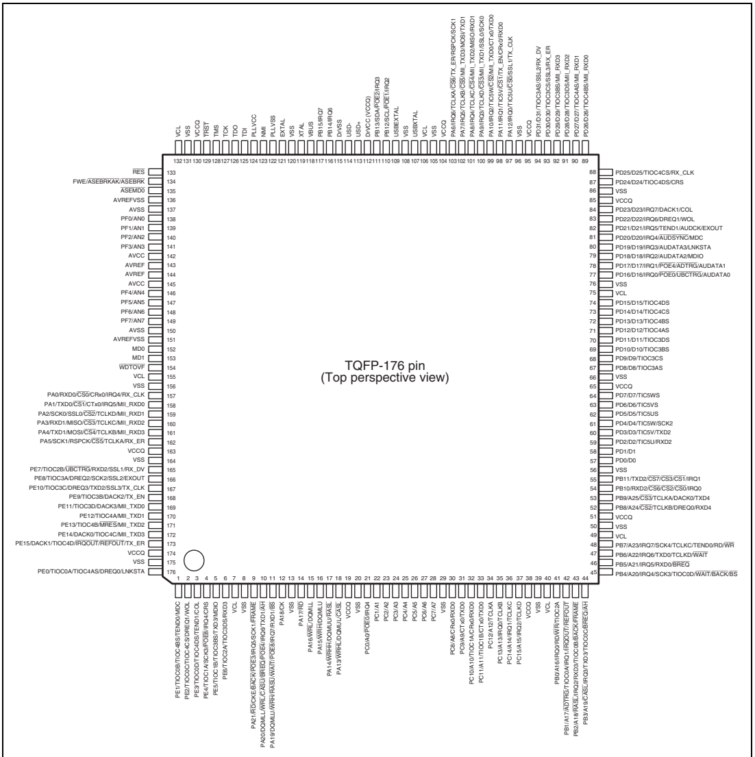
Figure 1.2 Pin Assignment (1)
