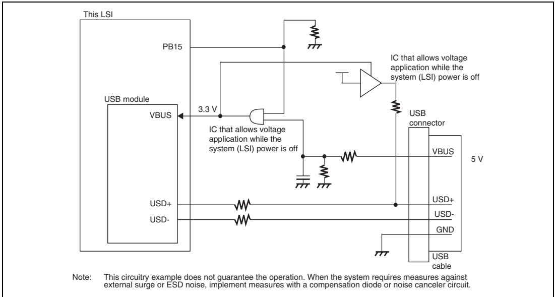
Figure 24.28 Example of USB Function Module External Circuitry
