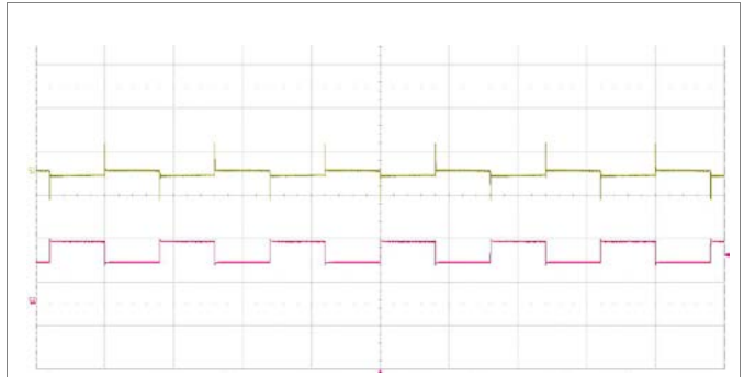
Output voltage response to load current step-change (5.0-7.5-5.0 A) at: T_{P1} = +25^{\circ}\text{C} , V_I = 24\text{ V} . Top trace: output voltage (500 mV/div.). Bottom trace: load current (5 A/div.). Time scale: (10 ms/div.).
