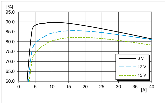
Efficiency vs. output current at T PI = +25°C
