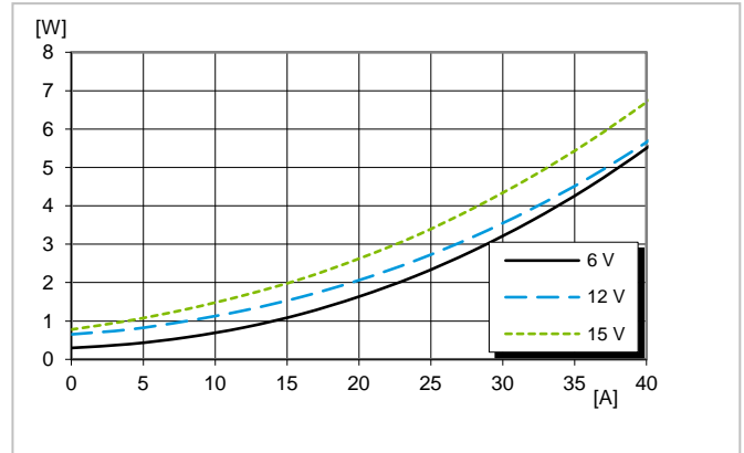
Dissipated power vs. load current at T PI = +25°C
