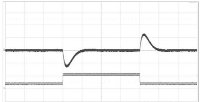
Output voltage response to output current change (7.5-22.5-7.5 A) at V_I=12\text{V} , C_o=5 \times 100 \mu\text{F} ceramic + 4 \times 470 \mu\text{F} POSCAP (ESR 10 m \Omega ), T_{PI} = +25^{\circ}\text{C} , di/dt=2\text{A}/\mu\text{s} .
