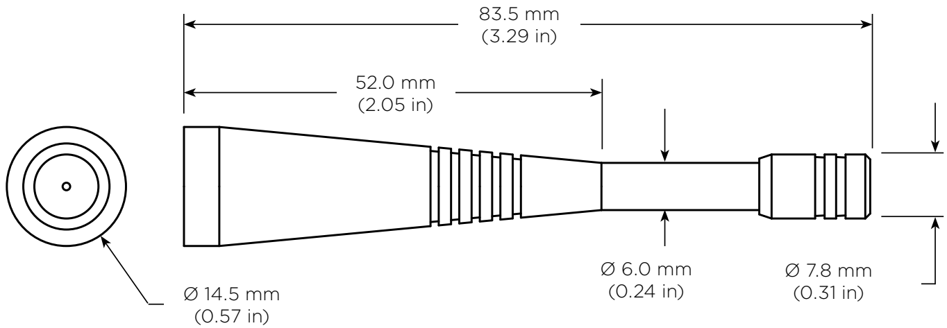
Figure 6: CW LTE Band 5 Antenna Dimensions
