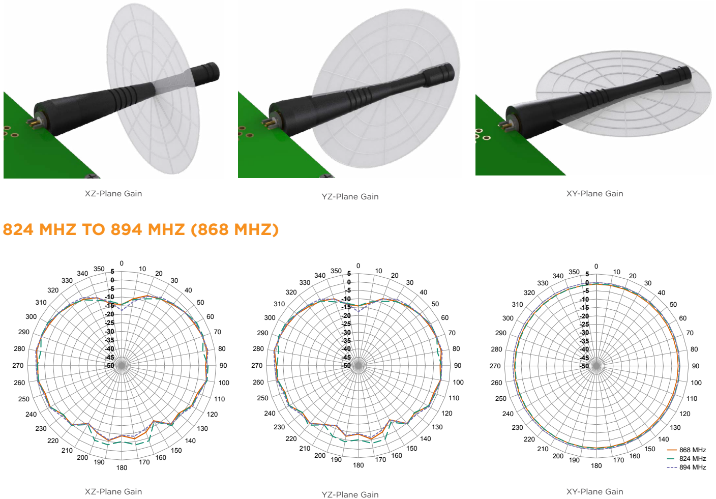
Figure 8: Radiation Patterns for CW LTE Band 5 Antenna
