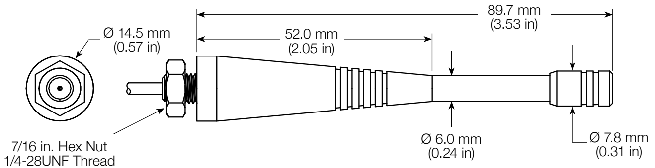
Figure 7: CW LTE Band 20 Antenna Dimensions
