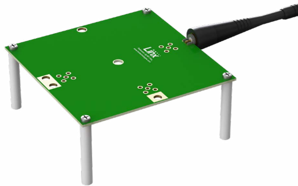
Figure 8: PW LTE Band 20 Antenna Shown On Edge of Evaluation Board
