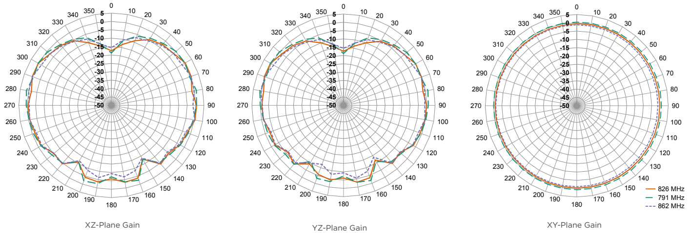
Figure 9: Radiation Patterns for PW LTE Band 20 Antenna
