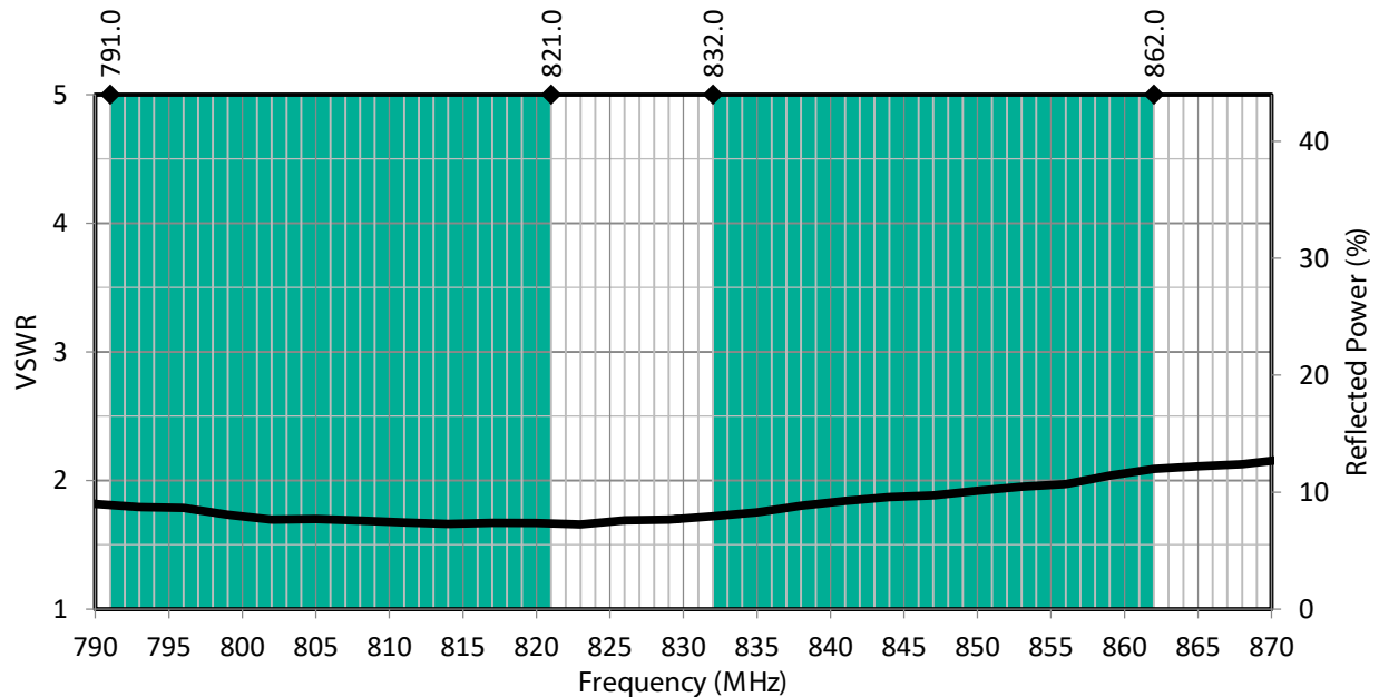
Figure 1: PW LTE Band 20 Antenna VSWR with Band 20 Uplink/Downlink Highlights
