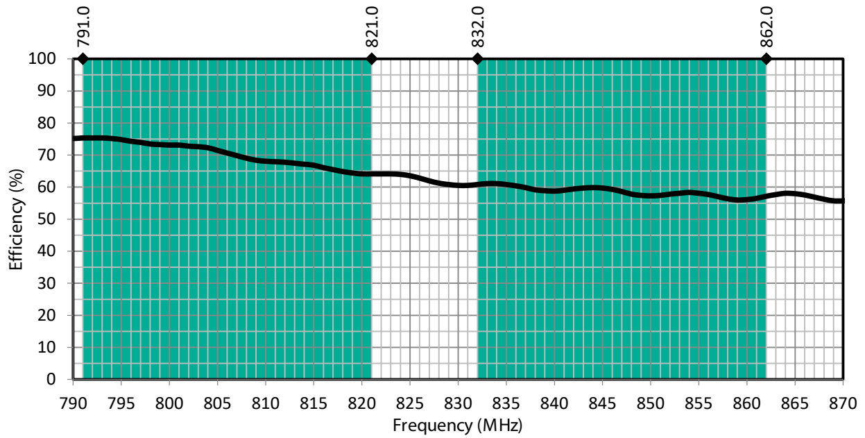
Figure 6: PW LTE Band 20 Antenna Radiation Efficiency with Band 20 Uplink/Downlink Highlights
