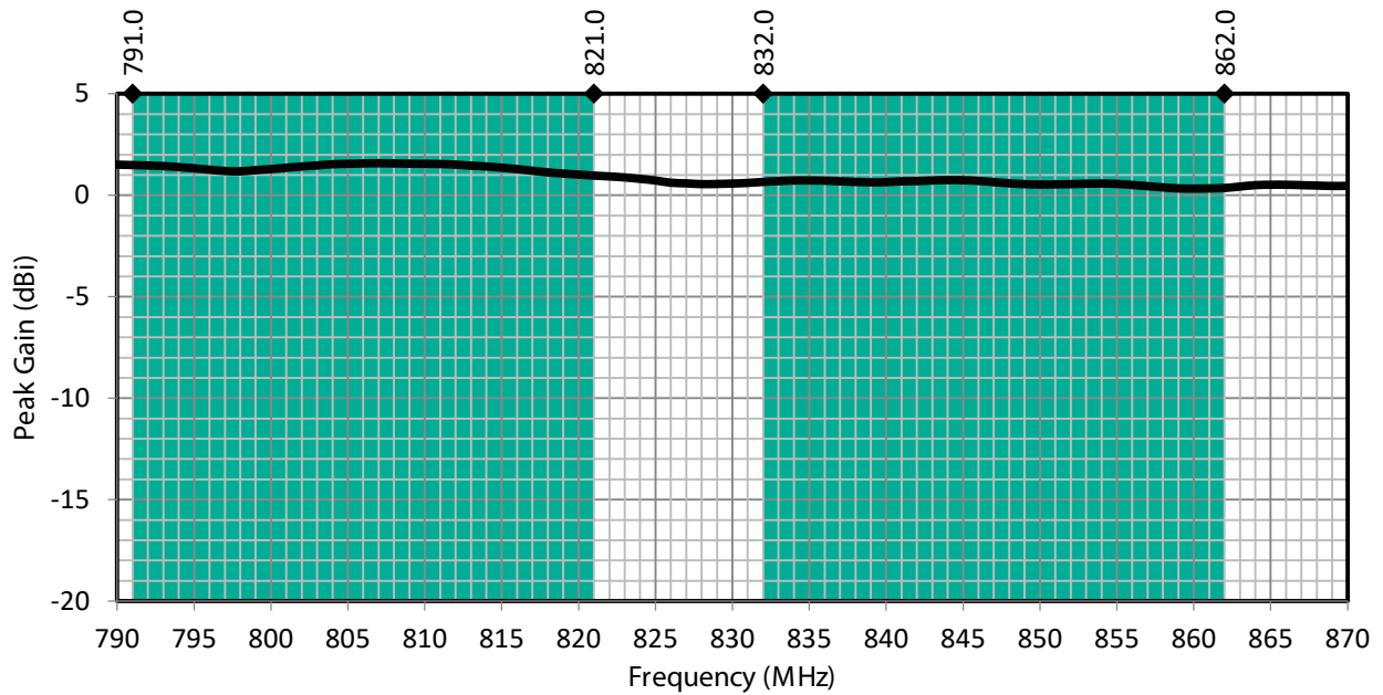
Figure 4: PW LTE Band 20 Antenna Peak Gain with Band 20 Uplink/Downlink Highlights
