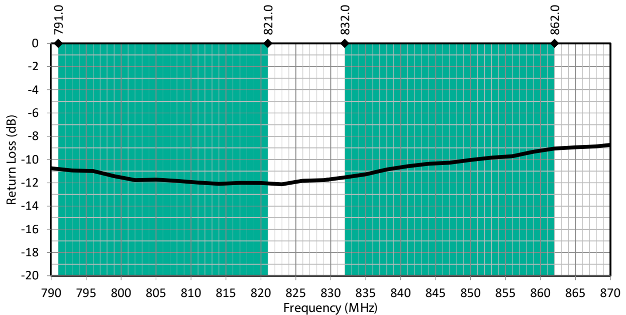
Figure 3: PW LTE Band 20 Antenna Return Loss with Band 20 Uplink/Downlink Highlights
