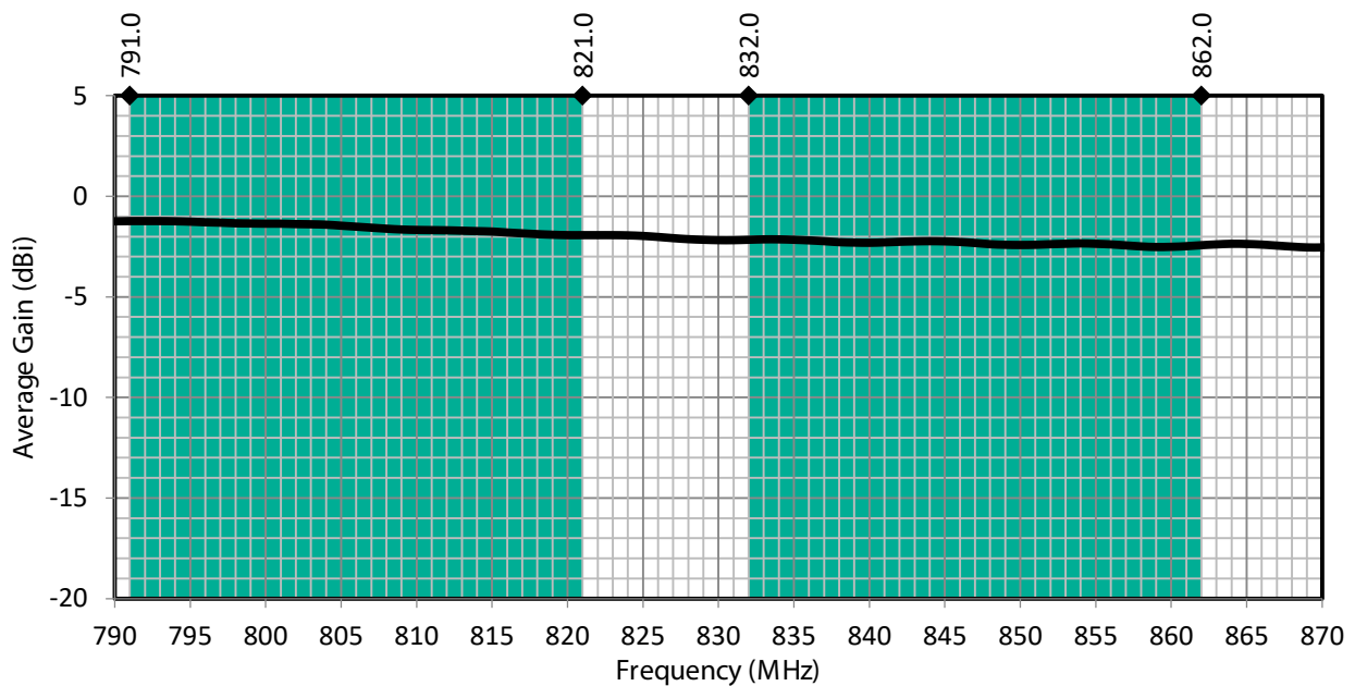
Figure 5: PW LTE Band 20 Antenna Average Gain with Band 20 Uplink/Downlink Highlights
