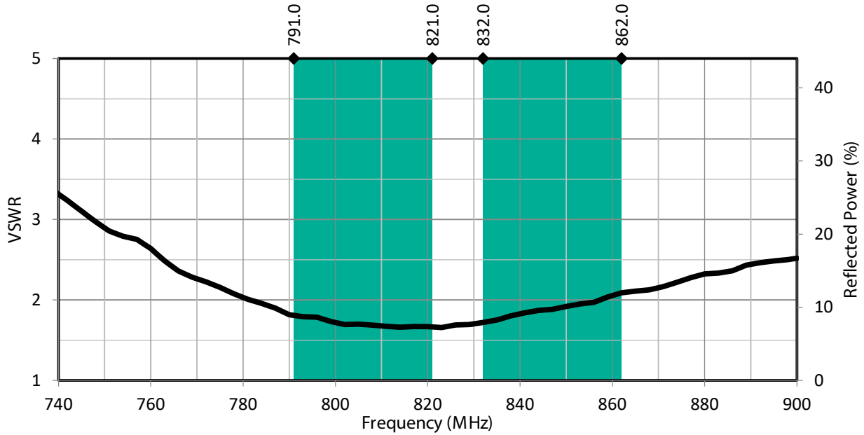
Figure 2: PW LTE Band 20 Antenna Full Bandwidth VSWR
