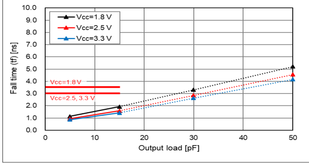
10% - 90% V CC , T use = +25 °C, Output load Char.
