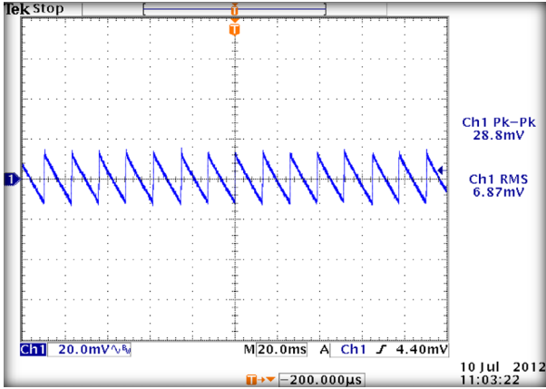
24V Out, No load, 90VAC, 60Hz
