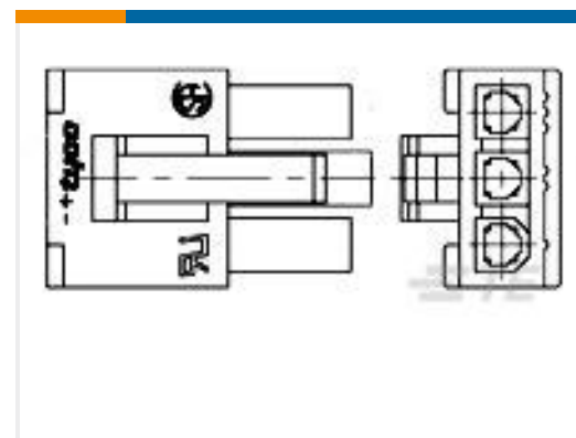
TE Part #1586027-5 5P SR RCPT VAL-U-LOK V0
