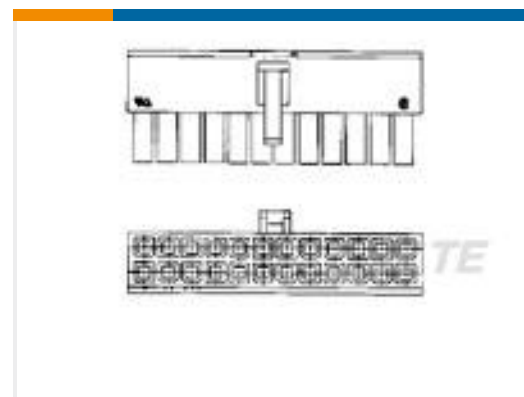
TE Part #1-1586765-0 10P RCPT VAL-U-LOK GW
