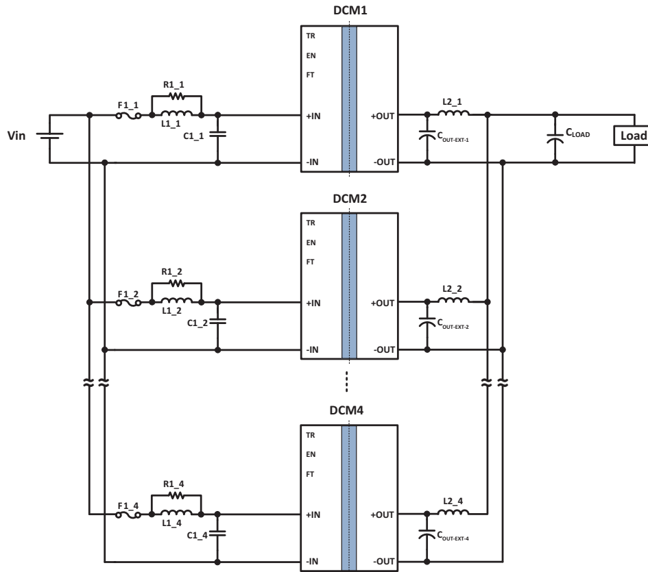
Typical Application 1: DCM3623xA5N06A2yzz in an array of four units
