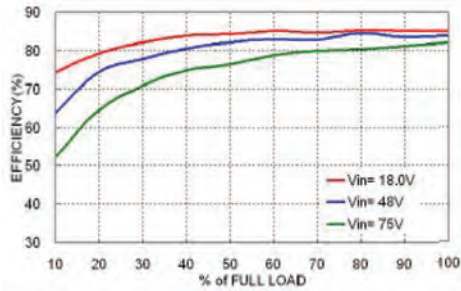
TWA3-48S5/MHIA5 Efficiency vs. Output Load
