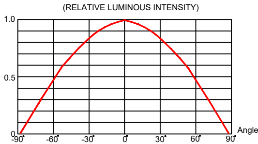
FIG.5 FAR FIELD PATTERN
