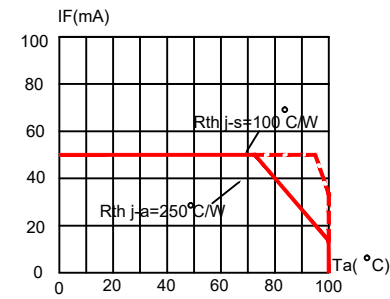
FIG.4 MAXIMUM FORWARD DC CURRENT VS AMBIENT TEMPERATURE (Tjmax=110°C)
