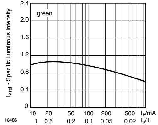
Fig. 16 - Relative Luminous Intensity vs. Forward Current/Duty Cycle
