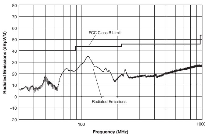
BWR-5/1700-D48A Radiated Emissions FCC Part 15 Class B, 3 Meters Converter Output = \pm 5Vdc @ \pm 1.6A
