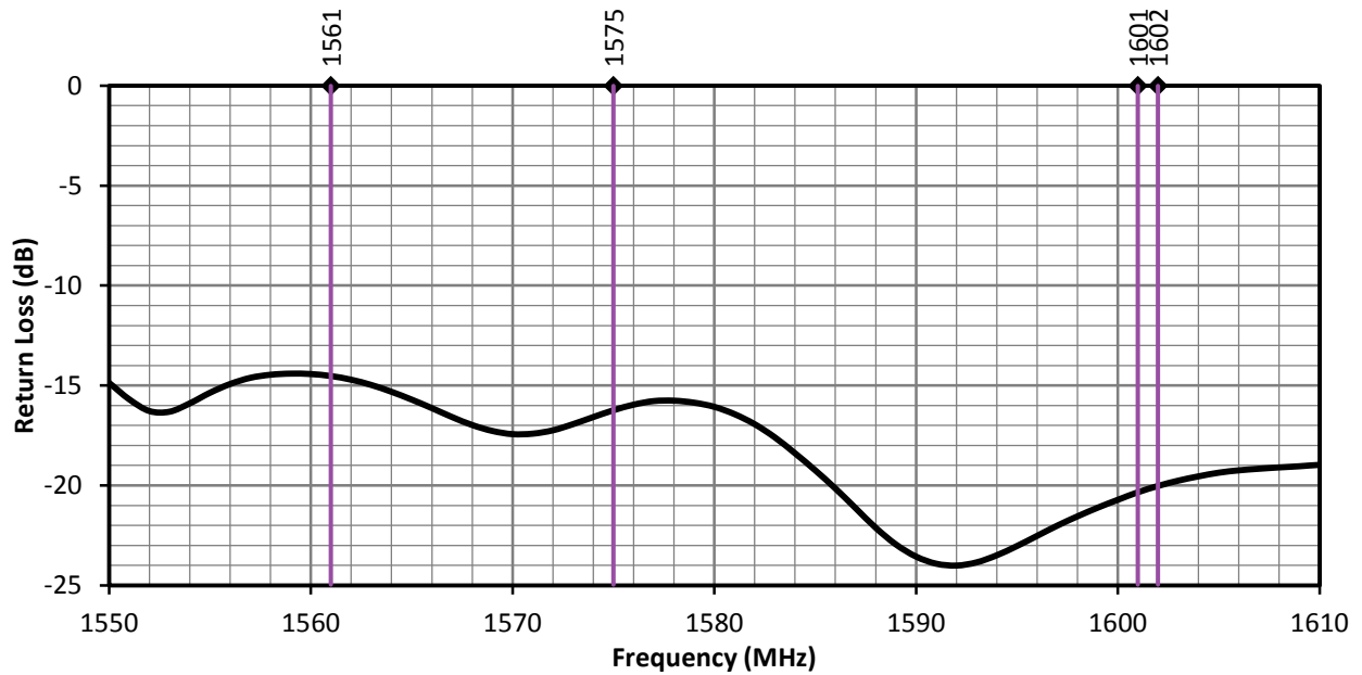
Figure 5. ANT-GNRM-L12A Series Antenna Return Loss, L1 Band
