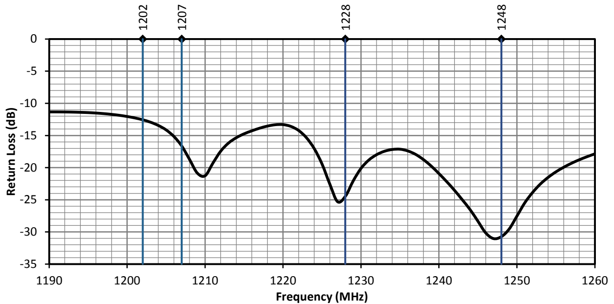
Figure 6. ANT-GNRM-L12A Series Antenna Return Loss, L2 Band
