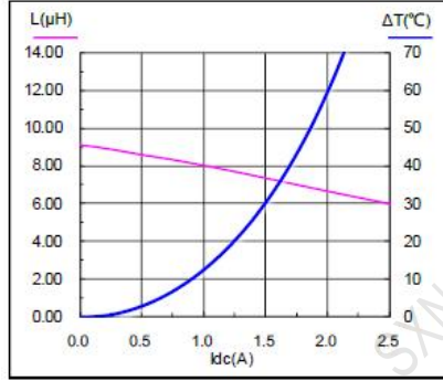
SMMS0420-100M
