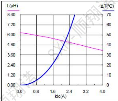
SMMS0420-6R8M
