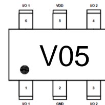
Marking Diagram
