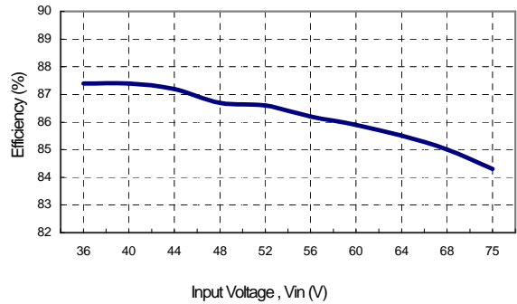
Efficiency versus Input Voltage. I o =Full Load
