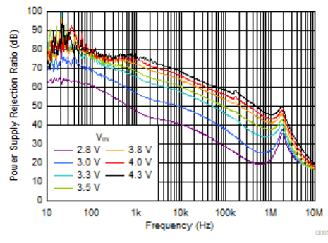
Figure 6-18. PSRR vs V_{IN}
