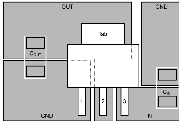
Figure 8-3. Layout Example
