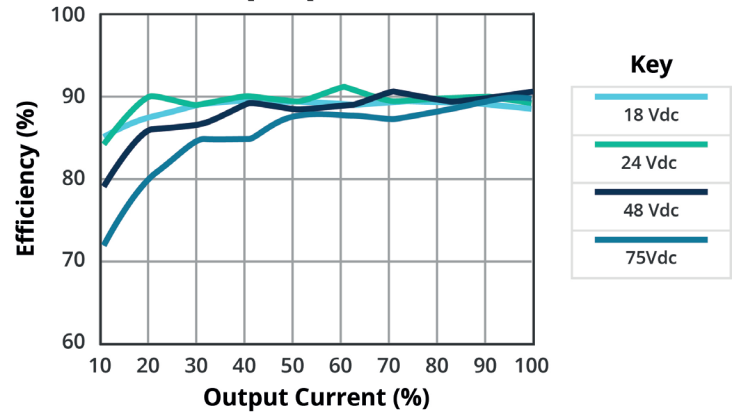
EFFICIENCY VS OUTPUT LOAD PDQ30-Q48-S15-D
