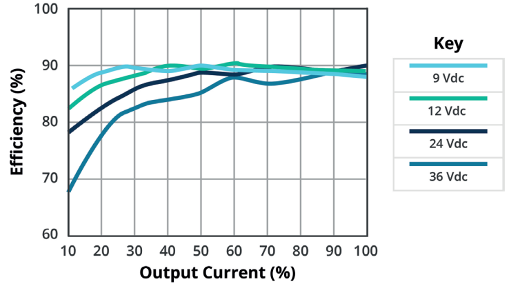
EFFICIENCY VS OUTPUT LOAD PDQ30-Q24-D15-D
