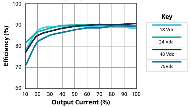
EFFICIENCY VS OUTPUT LOAD PDQ30-Q48-S5-D
