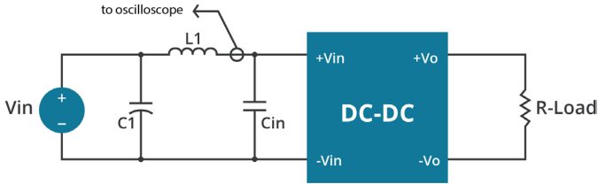
Figure 1 Measuring Input Ripple Current
