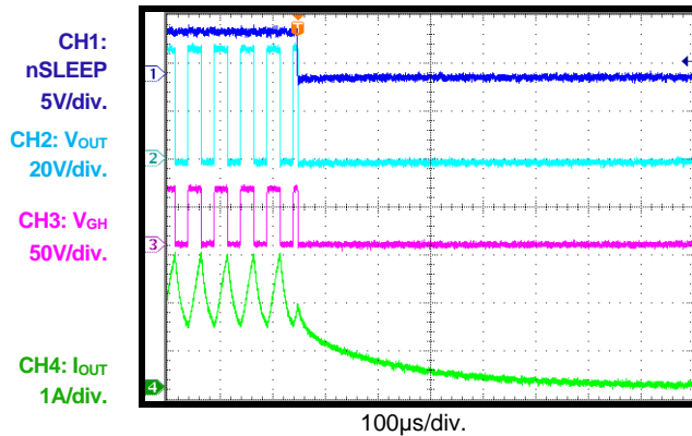
Sleep Mode Entry Duty = 50%
