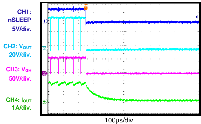
Sleep Mode Entry Duty = 90%, 30Ω + 2mH load
