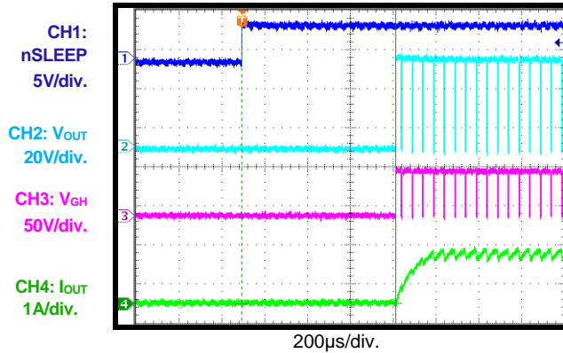
Sleep Mode Recovery Duty = 90%, 30Ω + 2mH load
