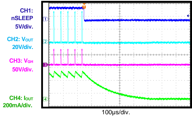
Sleep Mode Entry Duty = 10%
