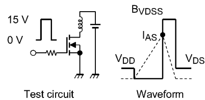
Fig. 9.16 Test Circuit/Waveform
