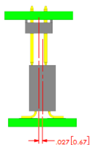
INITIAL Y AXIS LINEAR MISALIGNMENT
