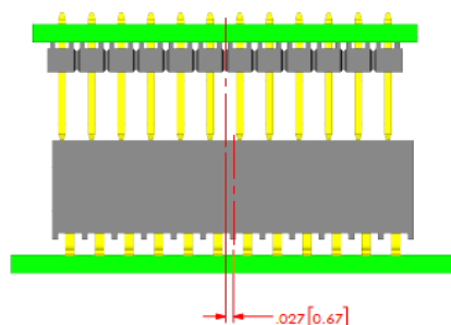
INITIAL X AXIS LINEAR MISALIGNMENT
