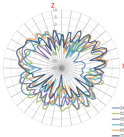
XZ Plane
