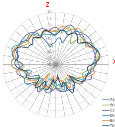
XZ Plane
