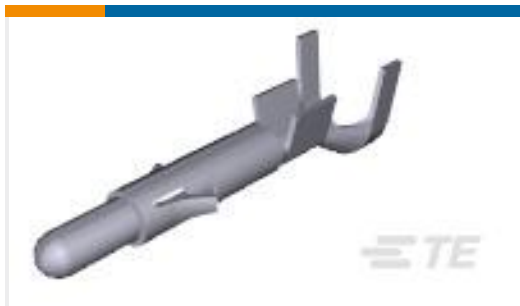
TE Part #350538-7 UMNL PIN 20-14 AU/NI/BR
