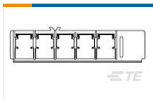
TE Part #5787590-1 BATT INT,INSERT ASSY,5P,7.2V
