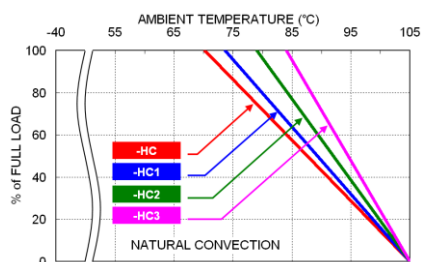
EED40-24S05W Derating Curve With Heat-sink
