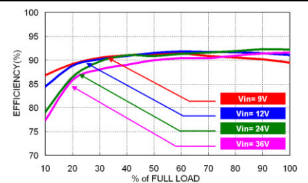
EED40-24S05W Efficiency vs. Output Load
