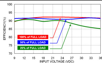
EED40-24S05W Efficiency vs. Input Voltage
