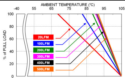
EED40-24S05W Derating Curve
