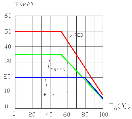
MAXIMUM FORWARD DC CURRENT VS, AMBIENT TEMPERATURE.
