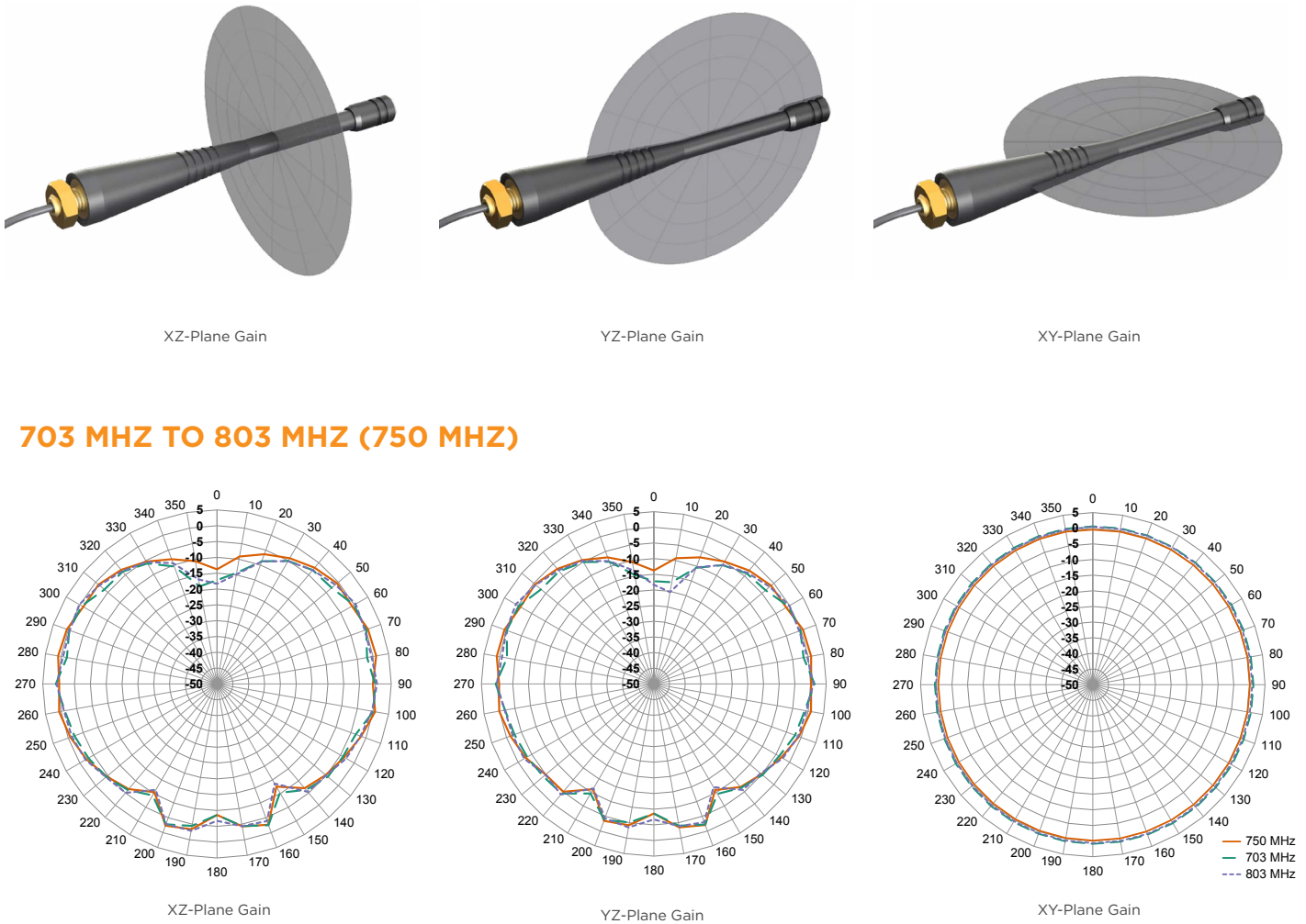
Figure 8: Radiation Patterns for PW LTE Band 28 Antenna
