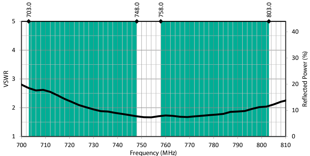
Figure 1: PW LTE Band 28 Antenna VSWR with Band 28 Uplink/Downlink Highlights
