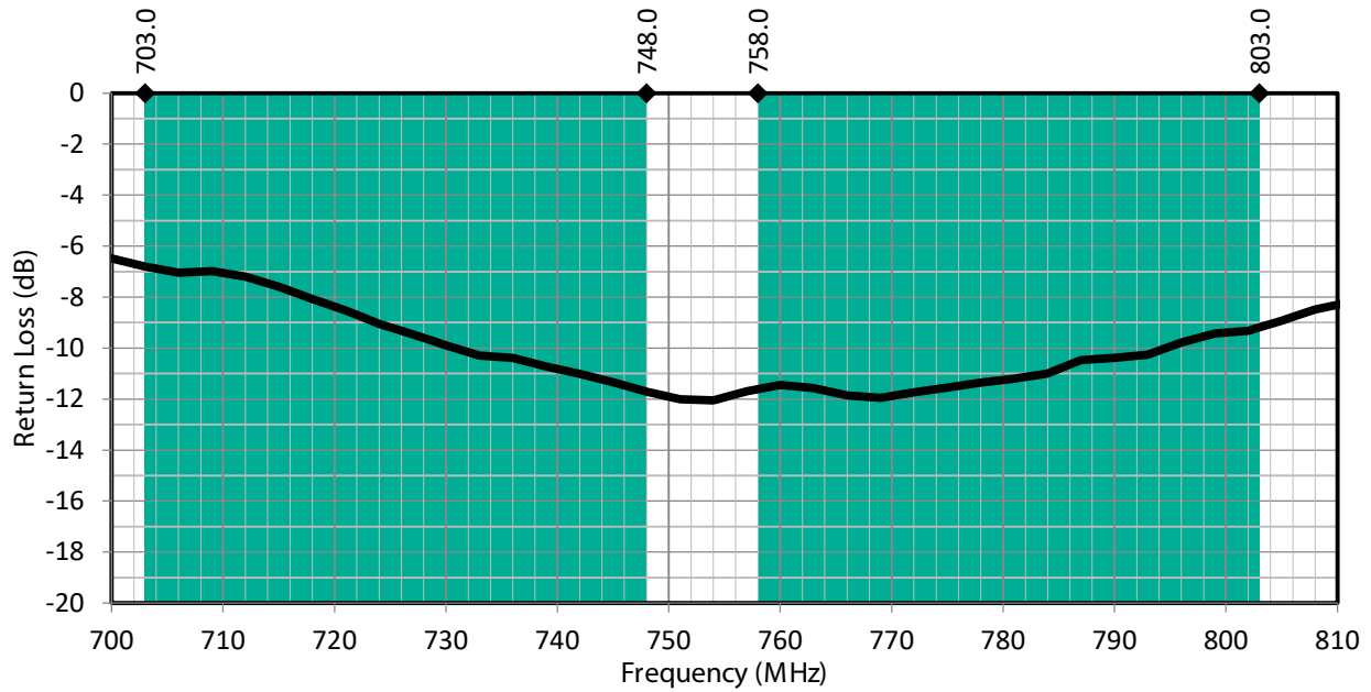
Figure 2: PW LTE Band 28 Antenna Return Loss with Band 28 Uplink/Downlink Highlights
