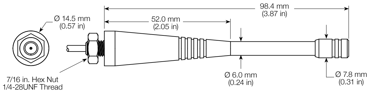
Figure 6: PW LTE Band 28 Antenna Dimensions
