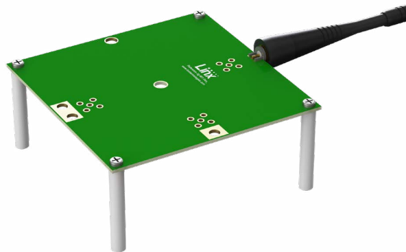
Figure 7: PW LTE Band 28 Antenna Shown On Edge of Evaluation Board
