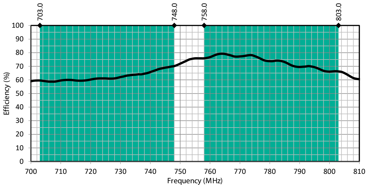
Figure 5: PW LTE Band 28 Antenna Radiation Efficiency with Band 28 Uplink/Downlink Highlights
