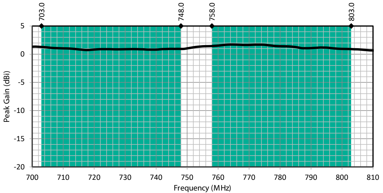
Figure 3: PW LTE Band 28 Antenna Peak Gain with Band 28 Uplink/Downlink Highlights
