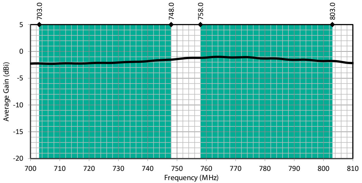
Figure 4: PW LTE Band 28 Antenna Average Gain with Band 28 Uplink/Downlink Highlights
