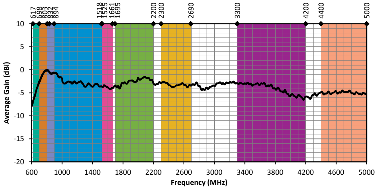
Figure 7. ANT-5GW-MMG2-SMA Antenna Average Gain on Ground Plane
