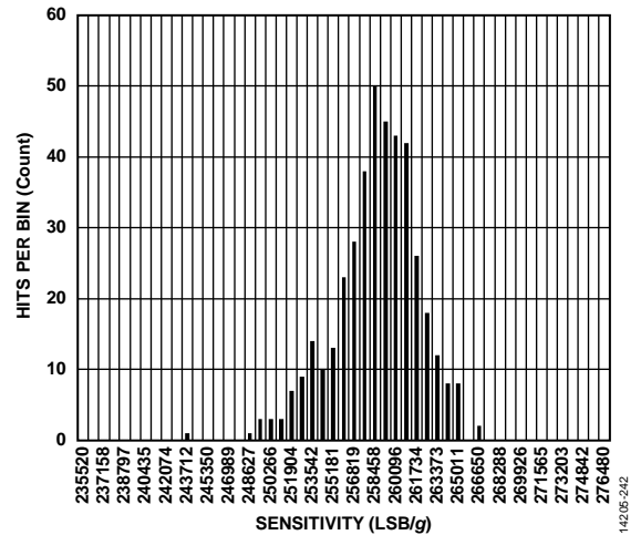
Figure 42. ADXL355 Sensitivity Histogram at 25°C, Z-Axis
