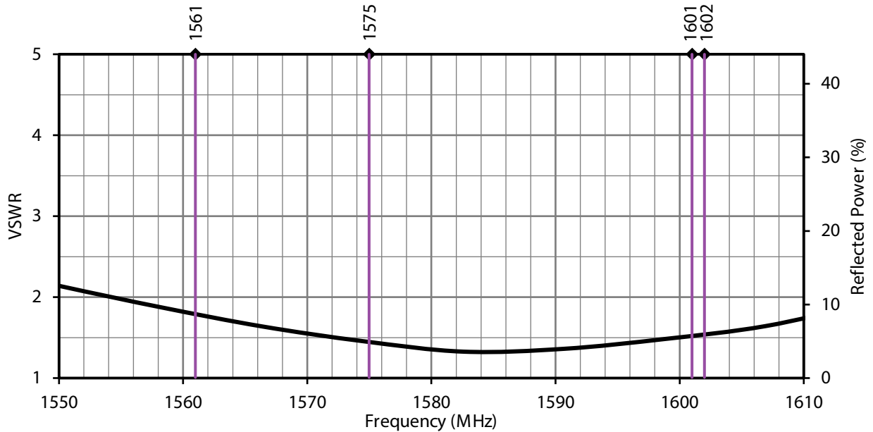
Figure 2. ANT-GNFPC-SHL1 Antenna VSWR with Frequency Band Highlights
