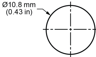
Figure 2. ANT-418-WRT Series Antenna Recommended Enclosure Mounting Dimensions
