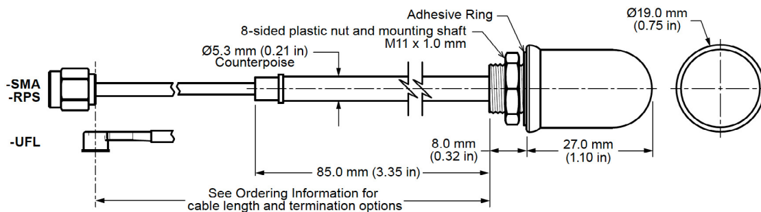
Figure 1. ANT-418-WRT Antenna Dimensions
