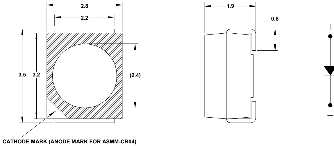
Figure 1: Package Drawing
