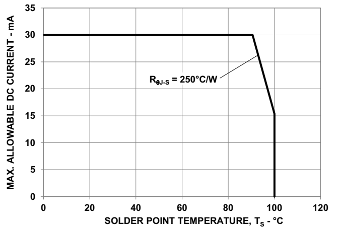
Figure 13: Maximum Forward Current vs. Solder Point Temperature - Red
