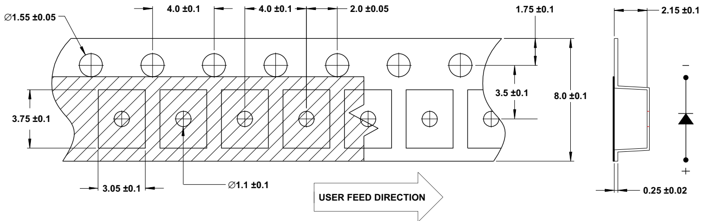
Figure 15: Carrier Tape Dimensions
