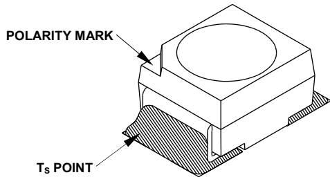
Figure 19: Solder Point Temperature on PCB
