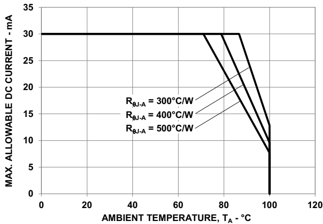
Figure 12: Maximum Forward Current vs. Ambient Temperature - Red
