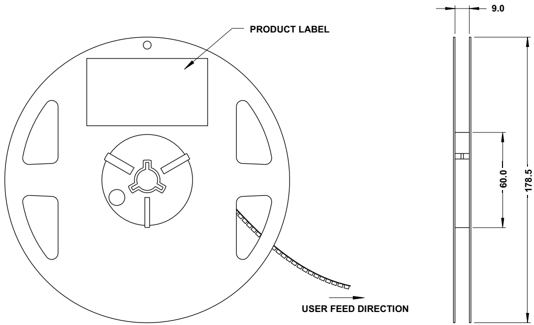
Figure 16: Reel Dimensions
