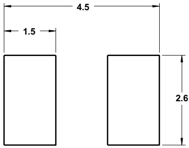
Figure 14: Recommended Soldering Land Pattern
