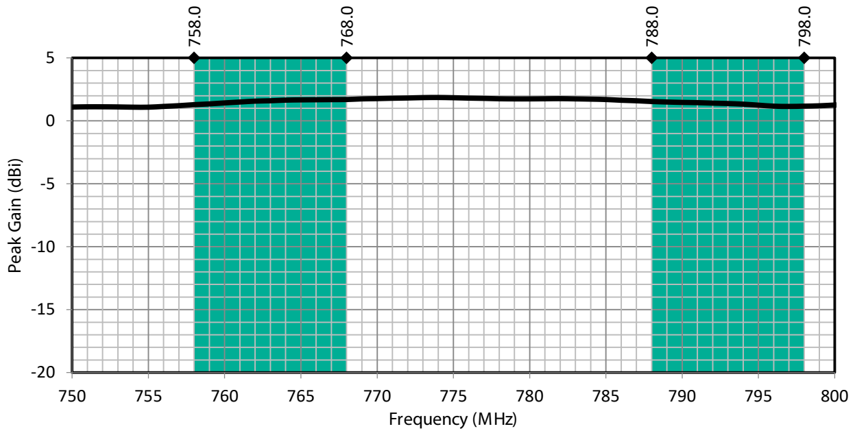
Figure 4: PW LTE Band 14 Antenna Peak Gain with Band 14 Uplink/Downlink Highlights
