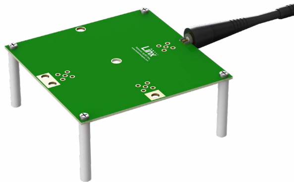
Figure 8: PW LTE Band 14 Antenna Shown On Edge of Evaluation Board
