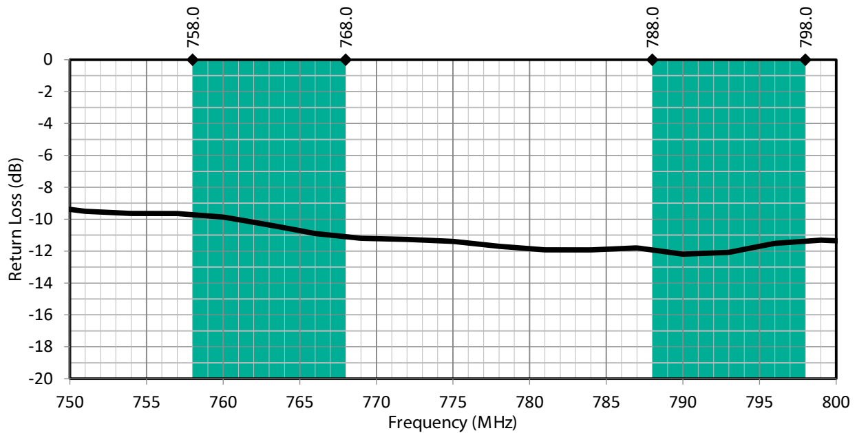
Figure 3: PW LTE Band 14 Antenna Return Loss with Band 14 Uplink/Downlink Highlights
