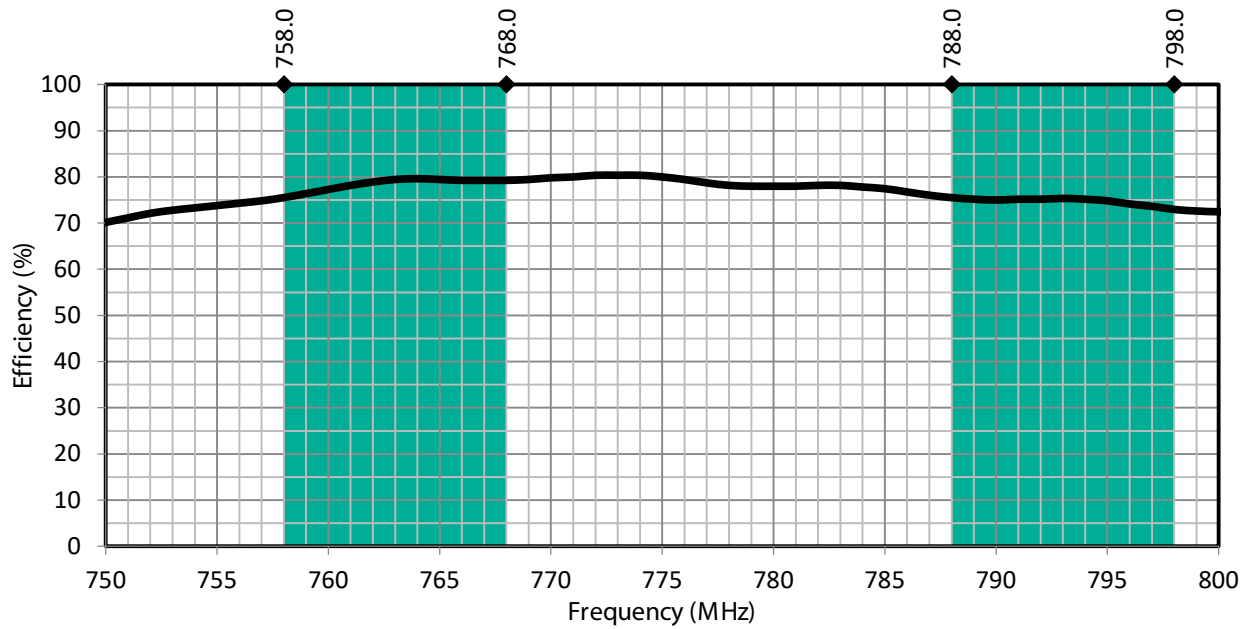
Figure 6: PW LTE Band 14 Antenna Radiation Efficiency with Band 14 Uplink/Downlink Highlights
