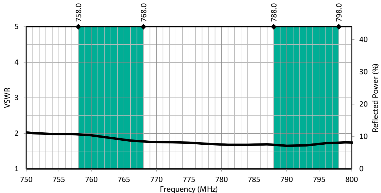
Figure 1: PW LTE Band 14 Antenna VSWR with Band 14 Uplink/Downlink Highlights
