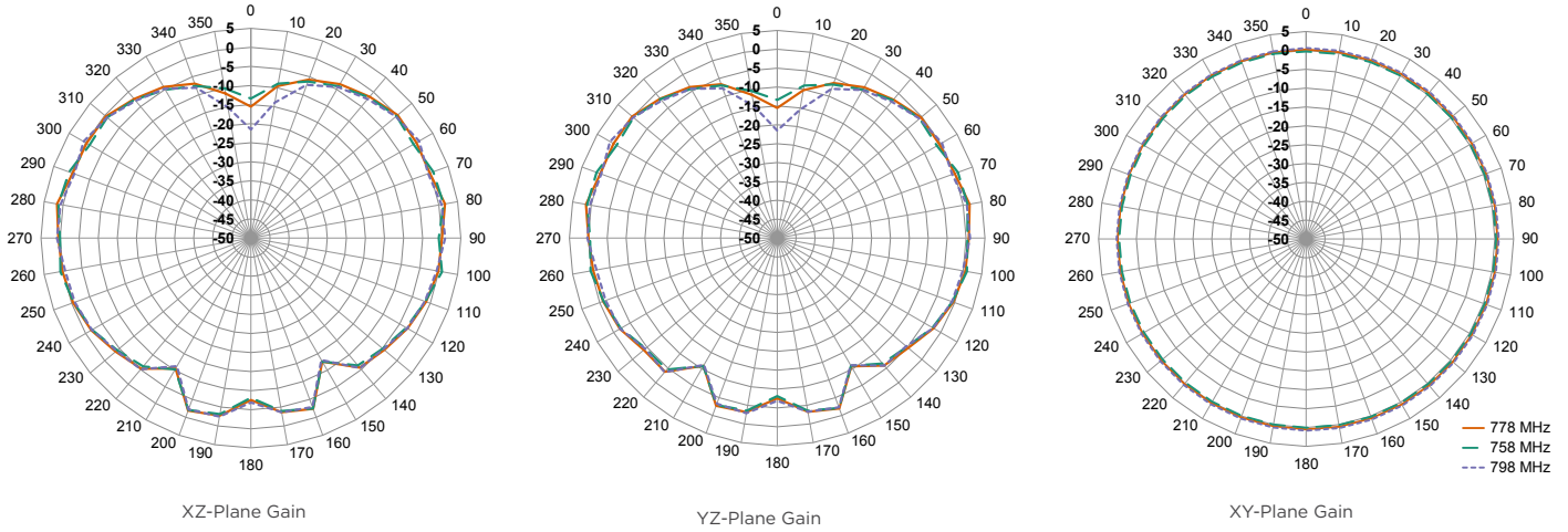
Figure 9: Radiation Patterns for PW LTE Band 14 Antenna
