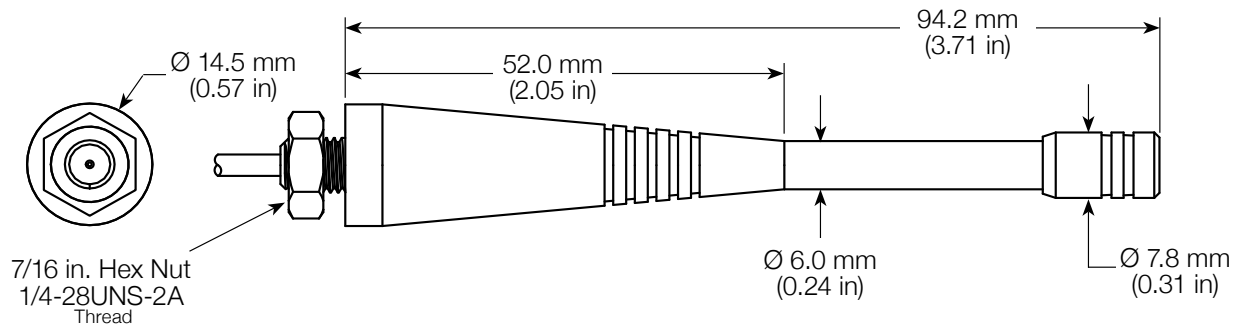
Figure 7: PW LTE Band 14 Antenna Dimensions
