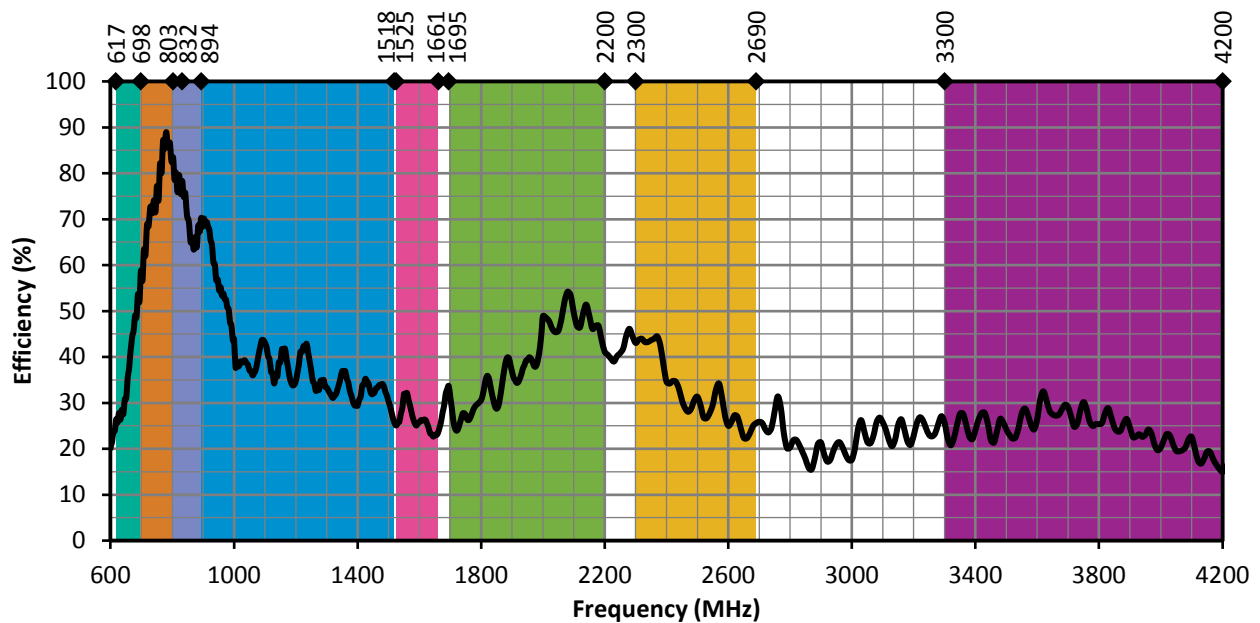
Figure 8. ANT-5GW-MMGI-SMA Antenna Efficiency on Ground Plane
