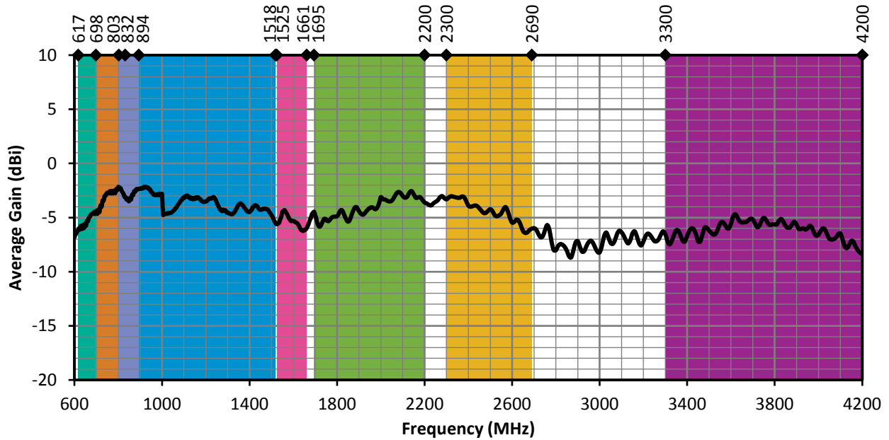
Figure 14. ANT-5GW-MMG1-SMA Antenna Average Gain, Free Space
