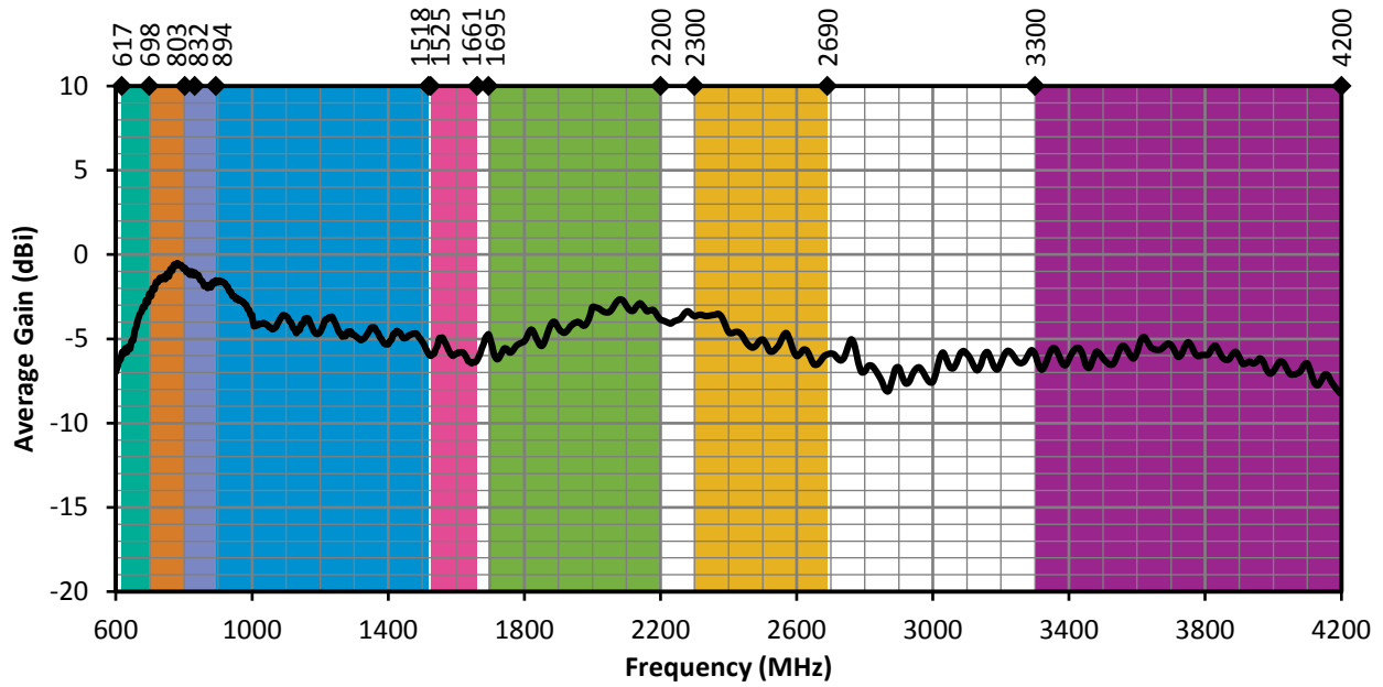
Figure 7. ANT-5GW-MMGI-SMA Antenna Average Gain on Ground Plane
